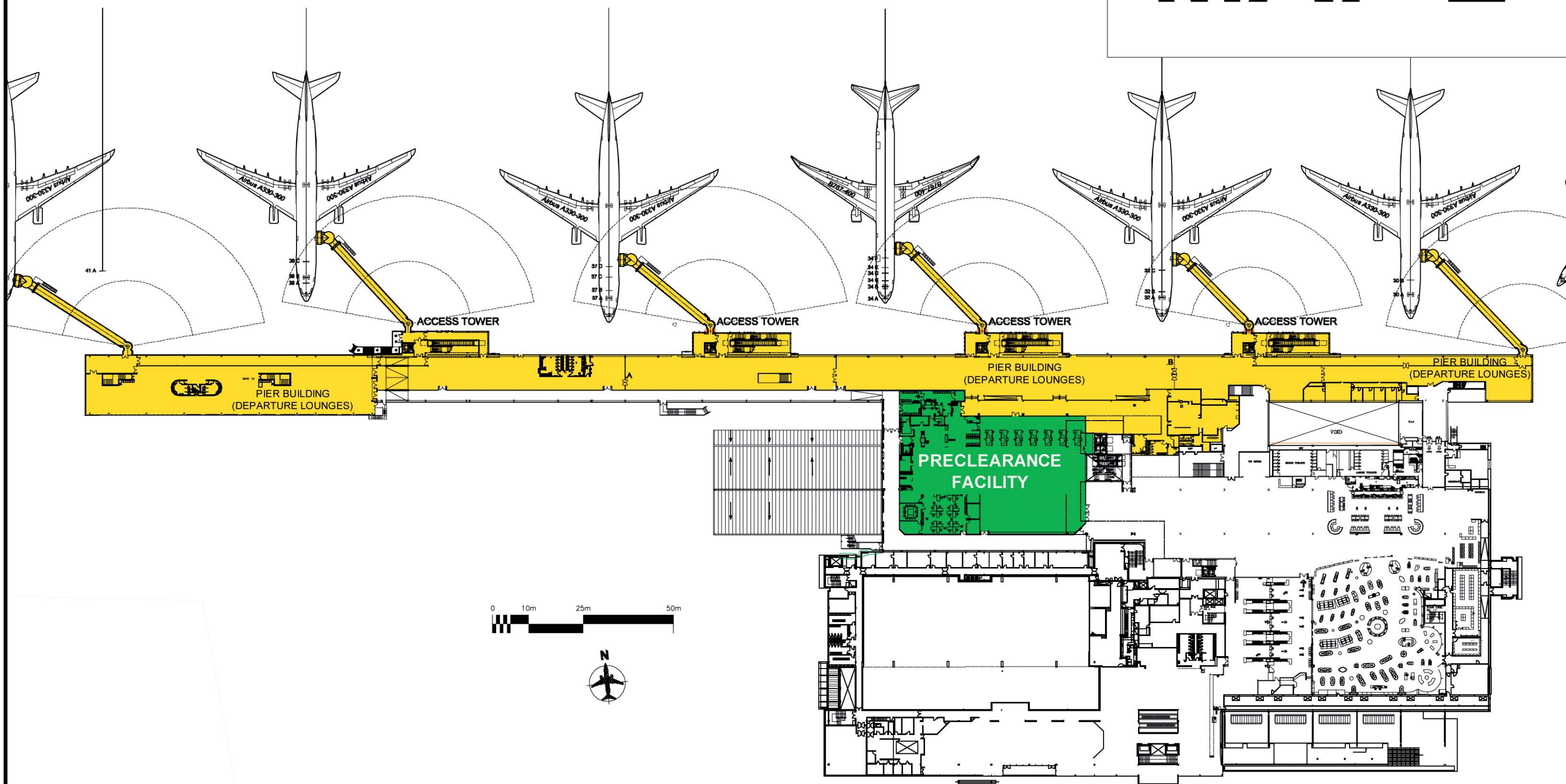
SHANNON AIRPORT TERMINAL FIRST FLOOR PLAN
